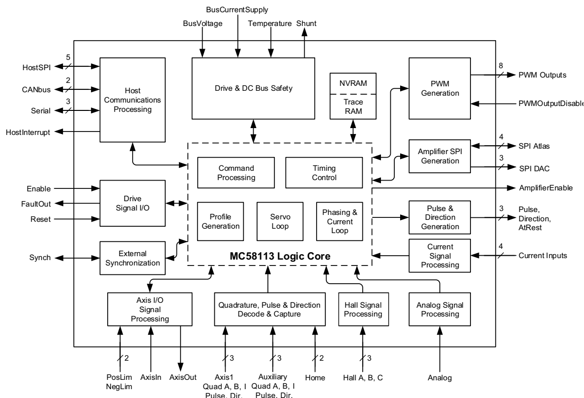
Figure 6-1: MC58113 Series ICs Internal Block Diagram
