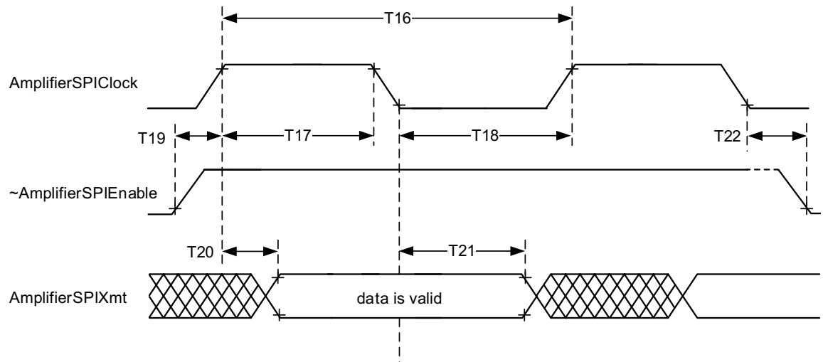
Figure 4-4: SPI DAC Timing
