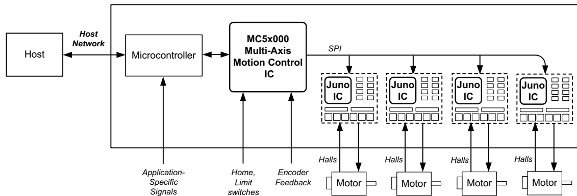
Figure 1-3: Multi-Axis Magellan Using On-Board Juno Torque Control ICs with Microcontroller
