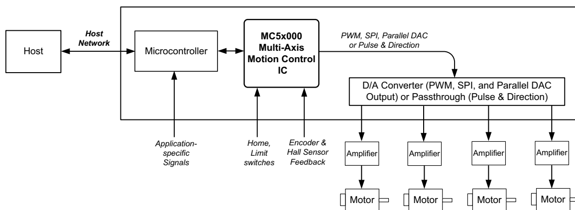
Figure 1-5: Multi-Axis Magellan Using Off-Board Amplifiers
